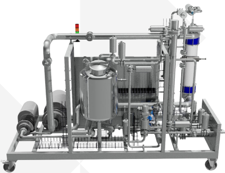
BMF-18 Compact S1 – Capacity 3-6 hl/h
